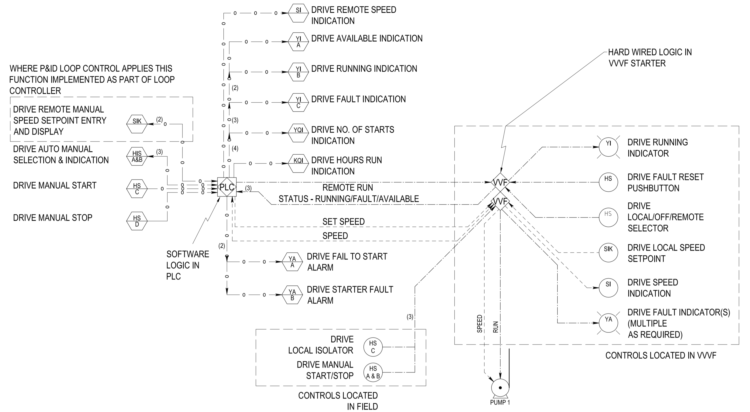
TYPICAL VARIABLE SPEED DRIVE MONITORING AND CONTROL
