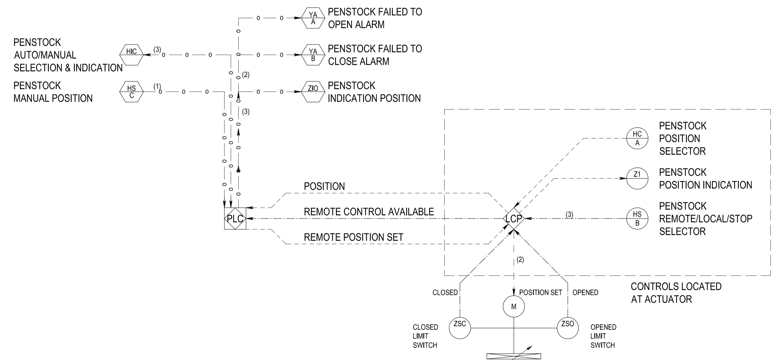
TYPICAL MODULATING PENSTOCK MONITORING AND CONTROL
