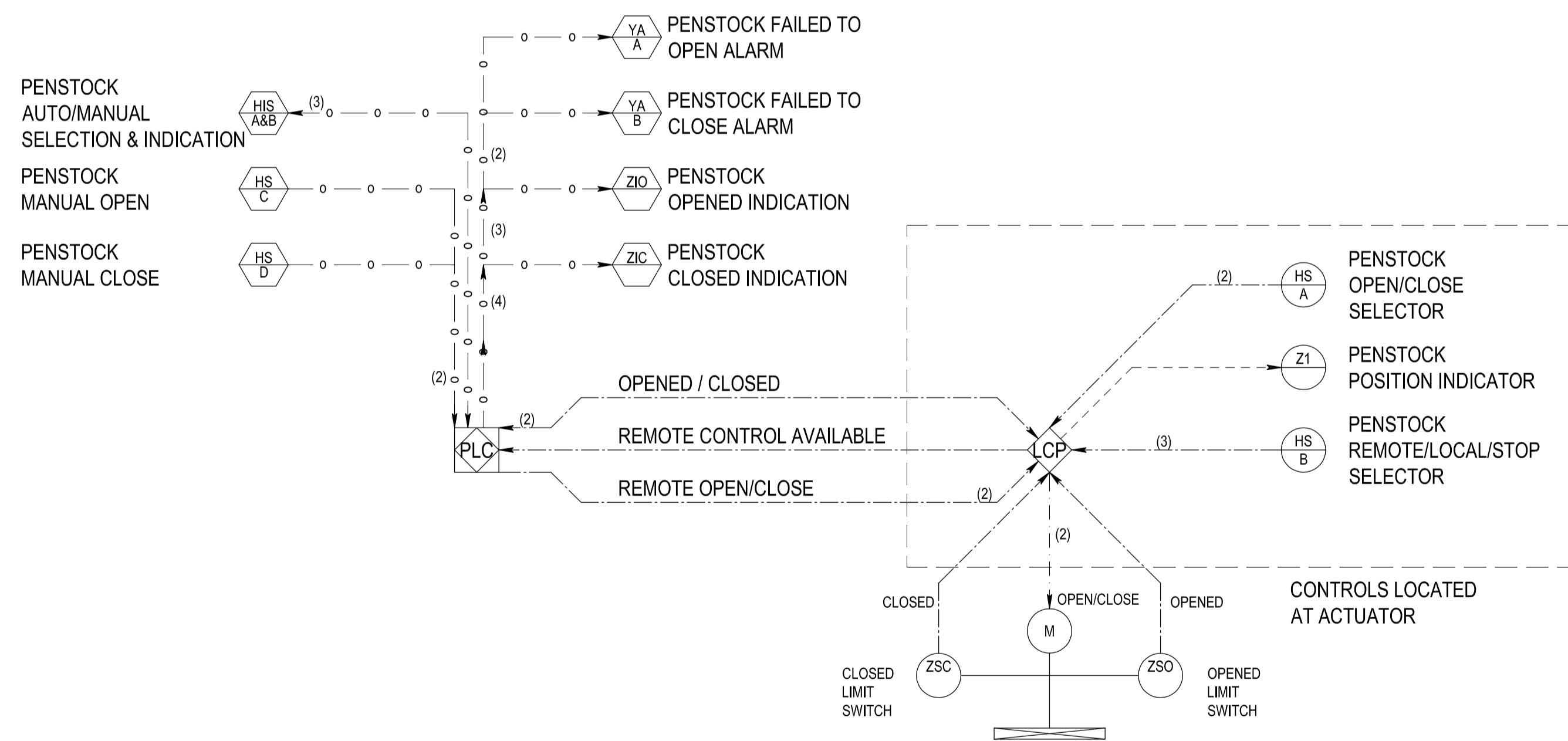
TYPICAL OPEN/CLOSE PENSTOCK MONITORING AND CONTROL
