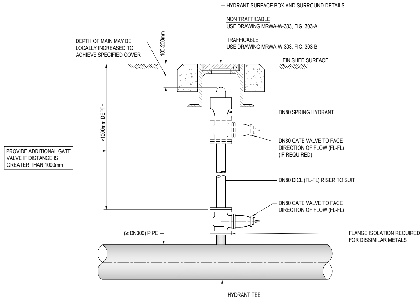
ELEVATION DN80 ISOLATING HYDRANT ASSEMBLY SCALE 1:10
